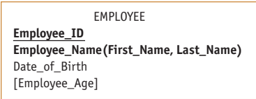
FIGURE 8-9 Required, optional, composite, and derived attributes
