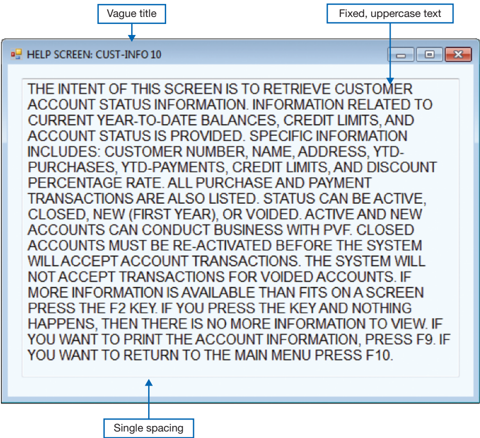
FIGURE 10-7 Contrasting the display of textual help information
